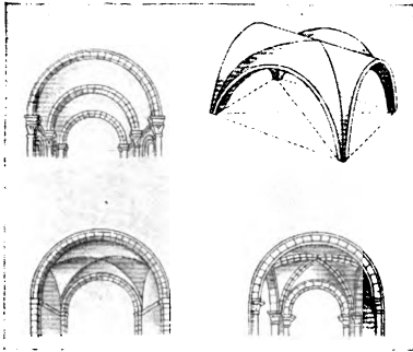
FIG. 161.—TYPES OF VAULTS.
